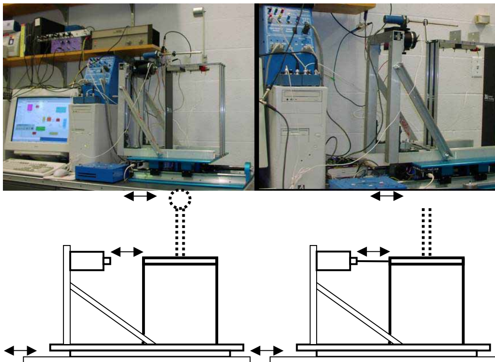
Figure 6. Small scale pilot testing of convolution method
