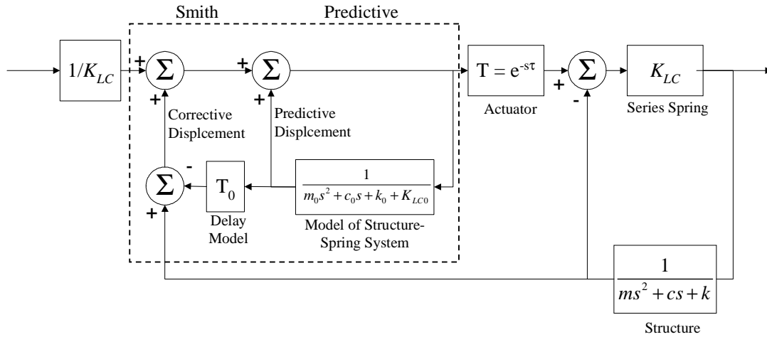
Figure 13. Smith predictive time-delay compensator
