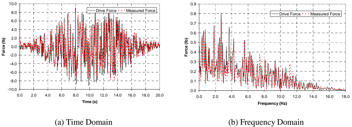
Figure 14. Target vs. achieved force in small-scale test
