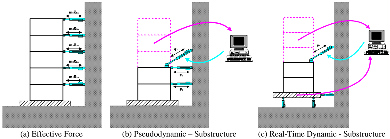
Figure 1. Modern Methods for “dynamic” testing in earthquake engineering.
