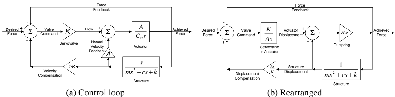
Figure 8. Force control of Dimig [6].
