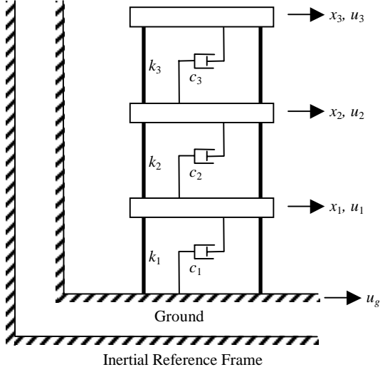
Figure 3. Three story model
