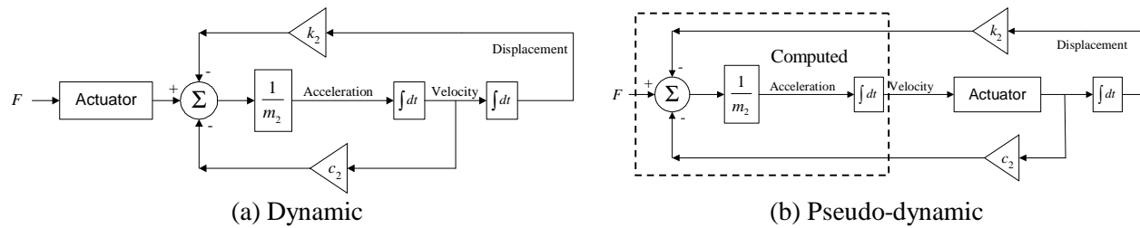
Figure 5. Dynamic and pseudo-dynamic testing
