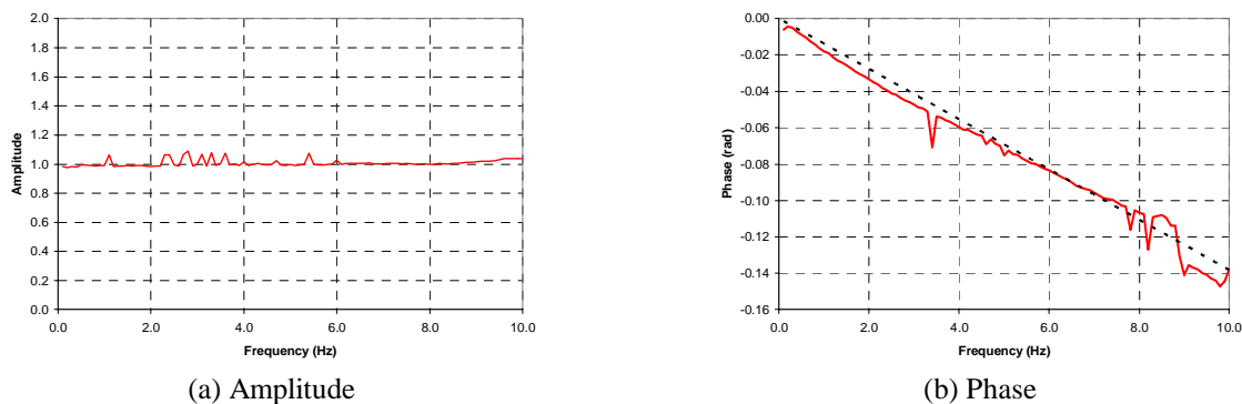
Figure 12. Actuator Transfer Function
