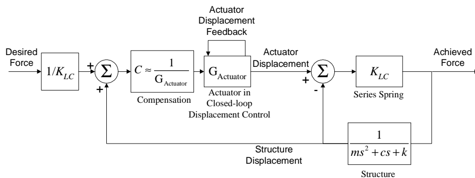
Figure 10. Block diagram of proposed force control
