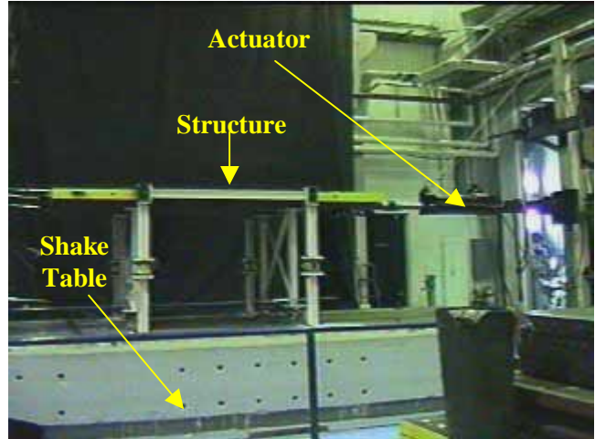
(b) Hybrid system –shake table and actuator
