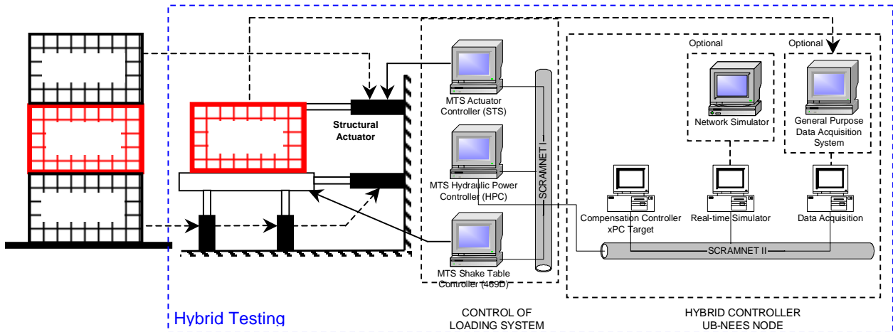
Figure 2. Schematic of Real-time Dynamic Hybrid Test System
