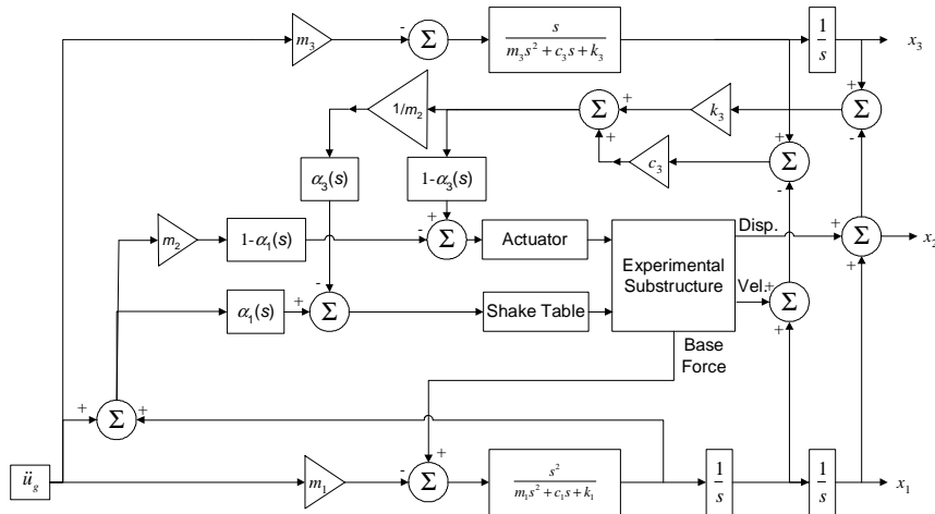
Figure 4. Schematic of hybrid substructuring
