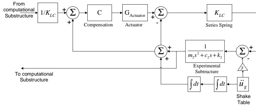
Figure 18. Control scheme for two story hybrid test
