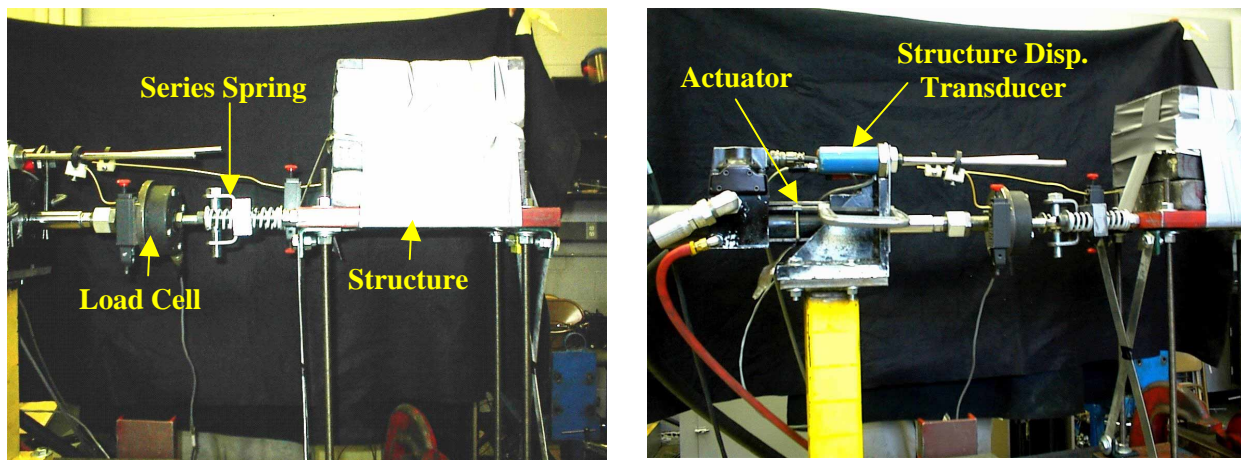
Figure 11. Small scale force control setup
