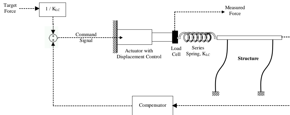
Figure 9. Proposed force control scheme
