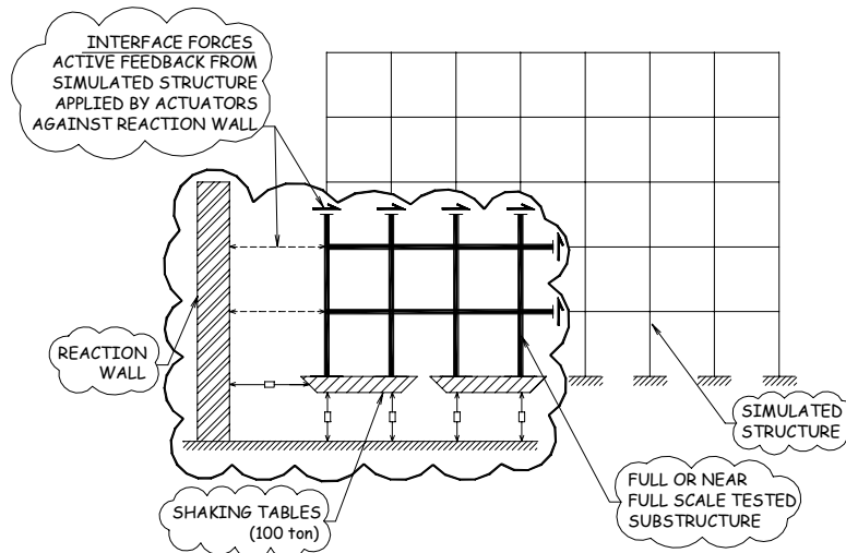
Fig.1. Real-Time Hybrid Seismic Testing System (Substructure Dynamic Testing)
